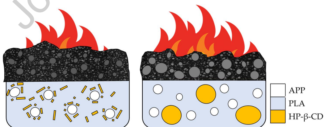
Figure 13 Schematic representation of the flame retardancy mechanism
