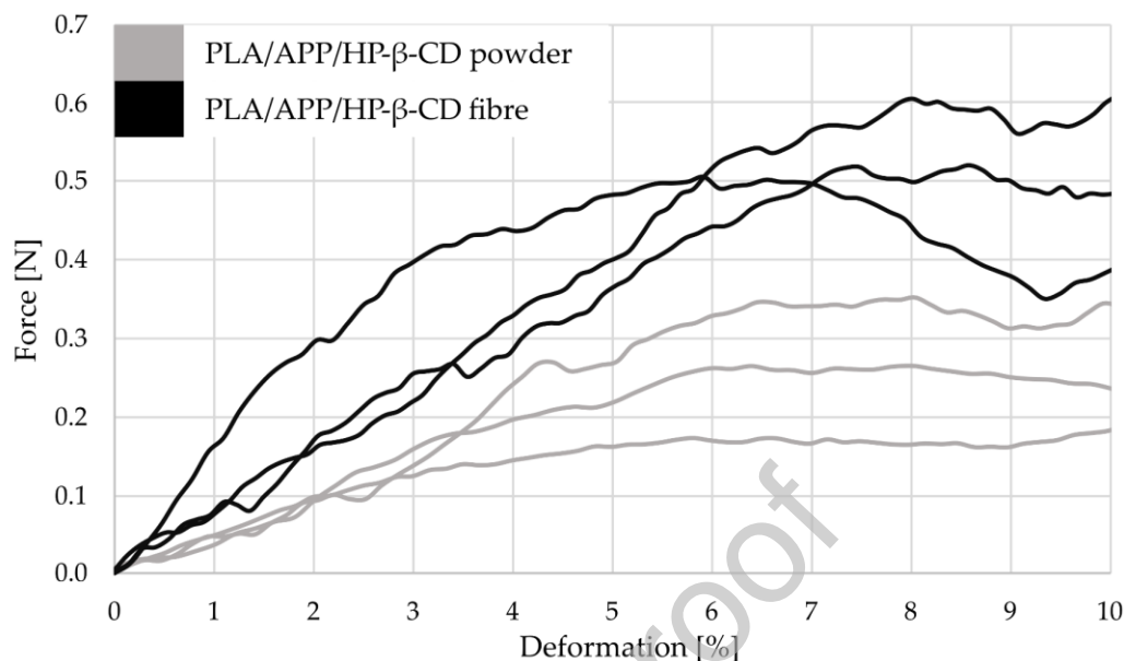
Figure 11 Normal force vs. deformation curves measured for the chars formed from the two types of HP- \beta -CD containing intumescent flame-retarded systems
