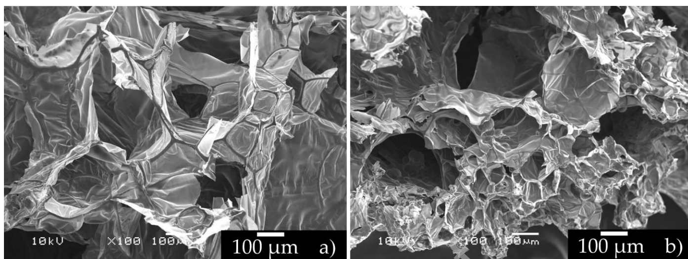
Figure 12 SEM images of the char residues; a) PLA/APP/HP- \beta -CD powder, b) PLA/APP/HP- \beta -CD fibre
