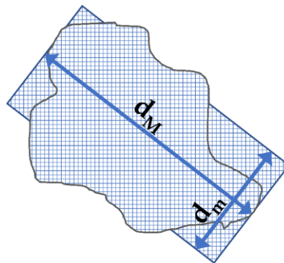
Figure 3 The estimation of the minimal diameter ( d_m ), the width of a rectangle with maximum diameter ( d_M ) length and the same area as the particle
