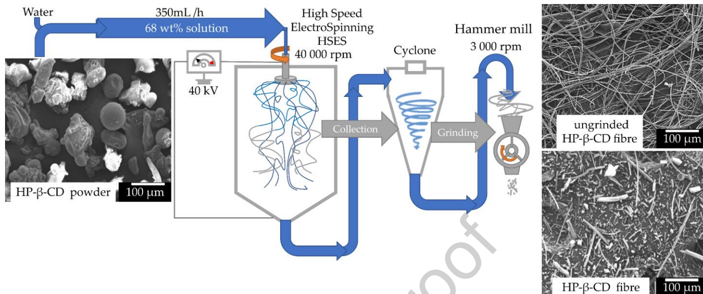
Figure 1 Preparation of the microfibrinous HP- \beta -CD additive
