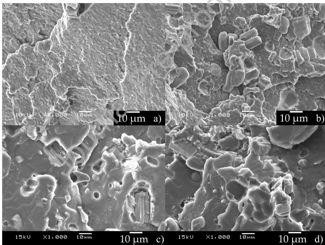
Figure 6 Scanning electron microscopic images of fracture surfaces with 1000 \times magnification: a) PLA, b) PLA/APP, c) PLA/APP/HP- \beta -CD powder and d) PLA/APP/HP- \beta -CD fibre.
