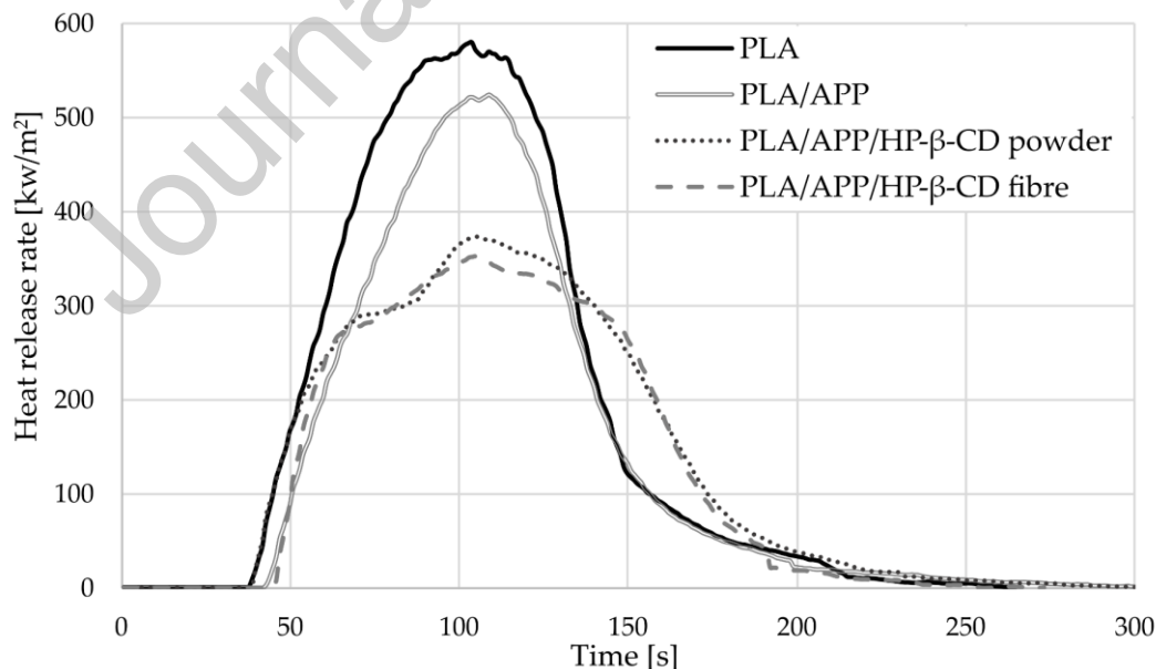
Figure 8 Heat release curves of polymer samples over time
