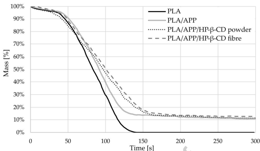
Figure 9 Mass loss of polymer samples over time
