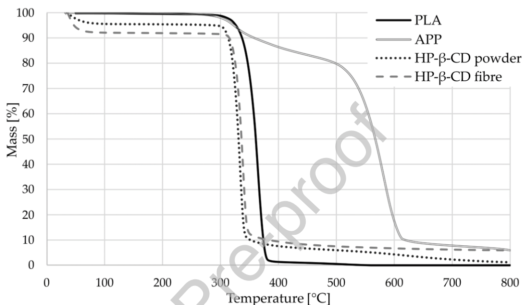
Figure 5 Thermogravimetric analysis (TGA) curves of poly(lactic acid) (PLA), APP and HP- \beta -CD powder and fibre additives as measured under N 2 atmosphere with the heating ramp of 10 °C/min.
