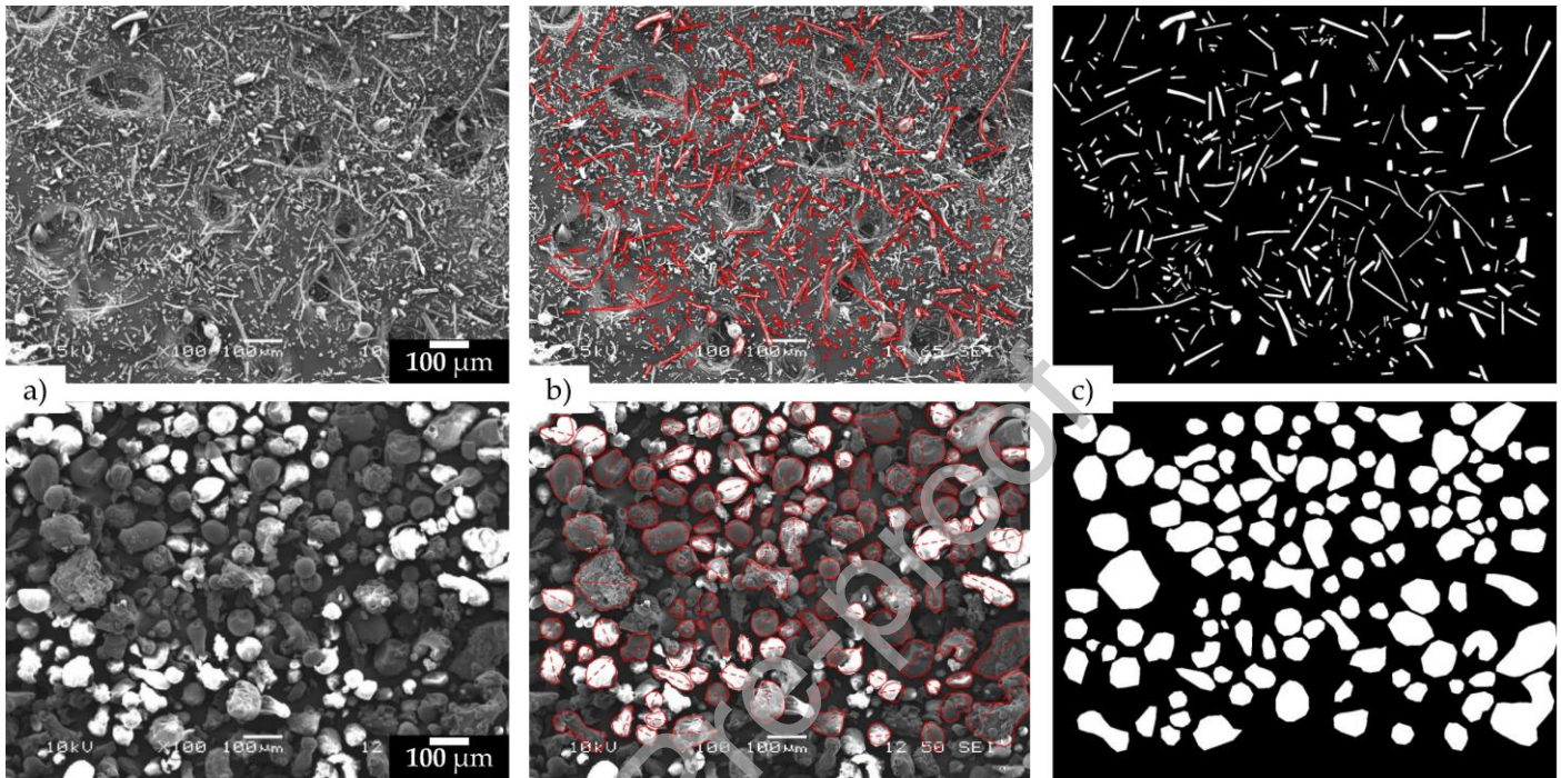
Figure 2 The steps of the particle size distribution measurement: (a) The SEM image, (b) the selected circumference of the particles and their maximum diameter (c) area of selected particles in the binary image.
