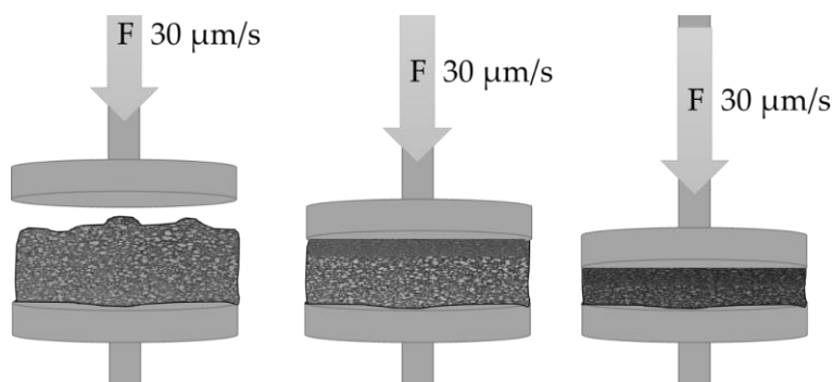
4. Figure Schematic representation of the char compression test
