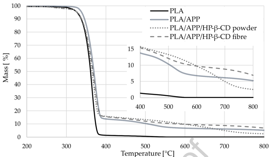
Figure 7 The thermogravimetric curves of the biopolymer composites (heating rate 10 °C/min, N 2 atmosphere).
