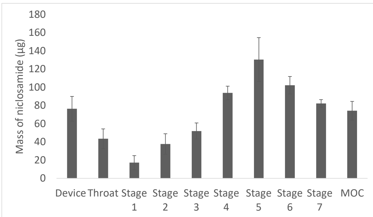
Figure 1. Aerodynamic particle size distribution of niclosamide inhalation powder ( n=3 ) made by thin-film freezing. The device bar indicates the remaining mass of niclosamide in the capsule and device. In the case of the throat bar, it indicates the remaining mass of niclosamide in the mouthpiece adapter and induction port.
