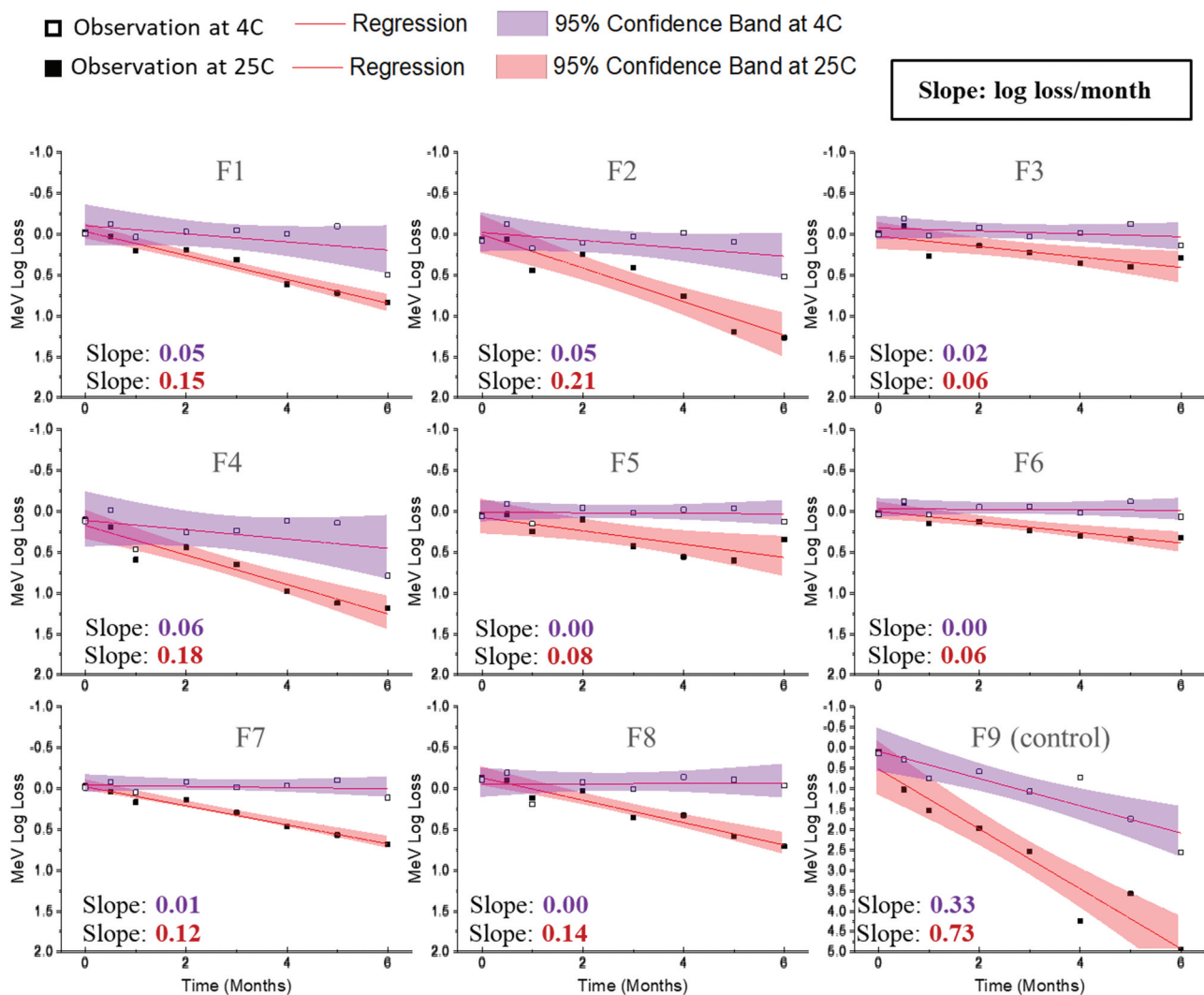
Figure 7. Stability profile of Me during accelerated ( 25^{\circ}\text{C} ) and real-time ( 2\text{--}8^{\circ}\text{C} ) stability studies with candidate MeRu formulations. Each candidate MeRu formulation was prepared, dried and then stored for 0.5, 1, 2, 3, 4, 5, and 6 months in the dried state. The in vitro potency of Me was measured by an infectivity RT-qPCR assay. \log_{10} loss values are relative to a control Me sample (frozen liquid bulk stored at -80^{\circ}\text{C} ). Solid lines (log loss/month) represent regression loss of Me viral titers (vs. control) and shaded bands represent 95% CI bands. Each titer was the average of quadruplicate measurements. See Figure 6 for composition of candidate MeRu formulations F1-F9.
