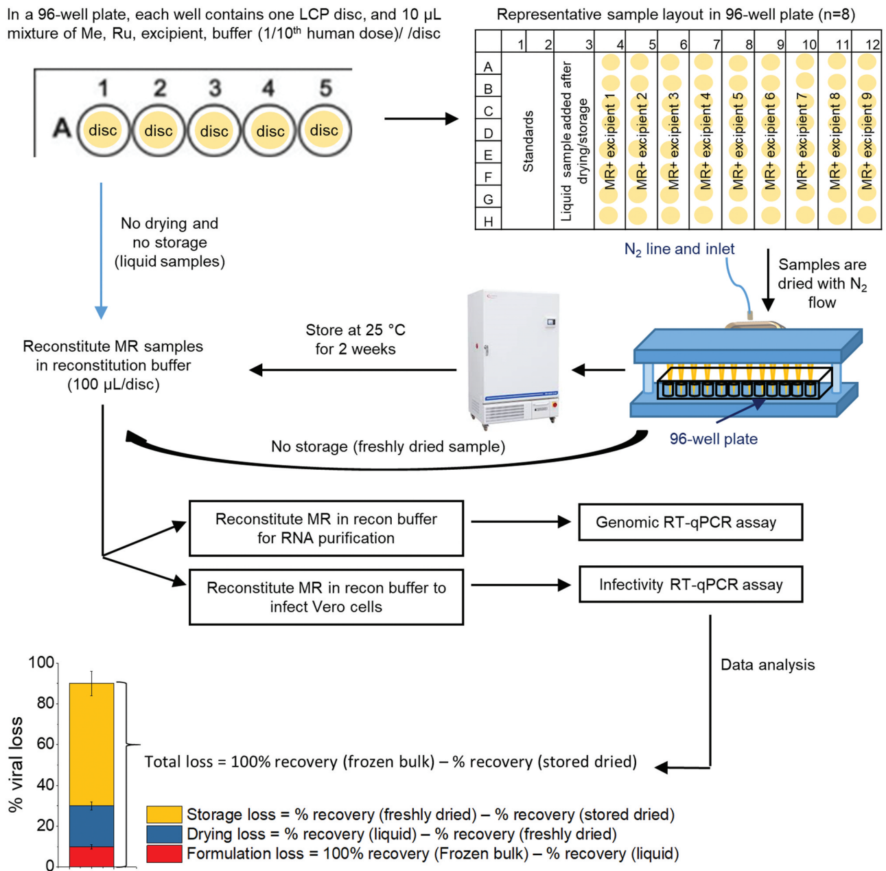
Figure 2. Overview of formulation experiments to assess the stability of Me and Ru (MeRu) viruses using a scaled-down lab model of Nanopatch TM coating/drying process. Flowchart shows the preparation of MeRu samples in various formulations at targeted titer of 10^{2.02} CCID 50 /disc for each virus (1/10 human dose), loading of samples into 96-well plates with LCP discs, drying by nitrogen, incubation of dried samples under various storage conditions, reconstitution of samples, and then determination of viral titers and genomes by infectivity and genomic RT-qPCR assays. The bottom panel shows the data analysis procedure to determine % losses of viral titers and viral particles during formulation, drying and storage. The values of each sample were normalized to frozen bulk stored at -80^{\circ} C (100%).
